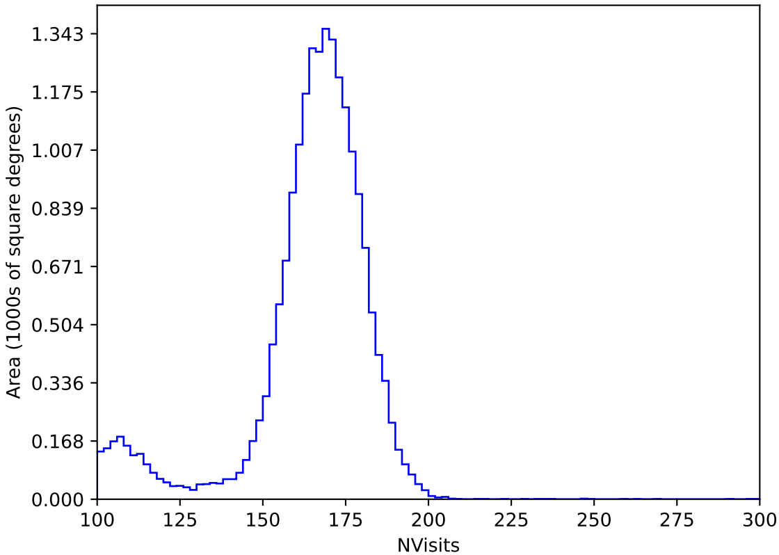
ddf_loaded_half_fl4_v3.4_10yrs All sky y band: NVisits
