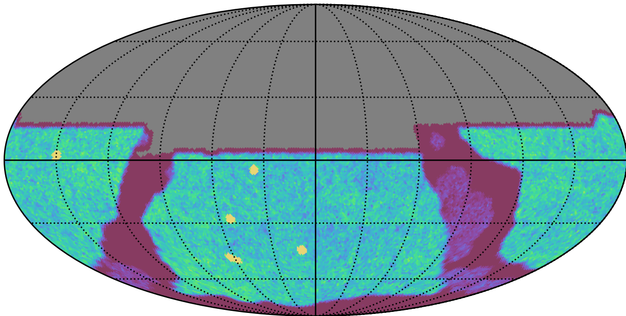
ddf_loaded_half_fl4_v3.4_10yrs All sky u band: NVisits
