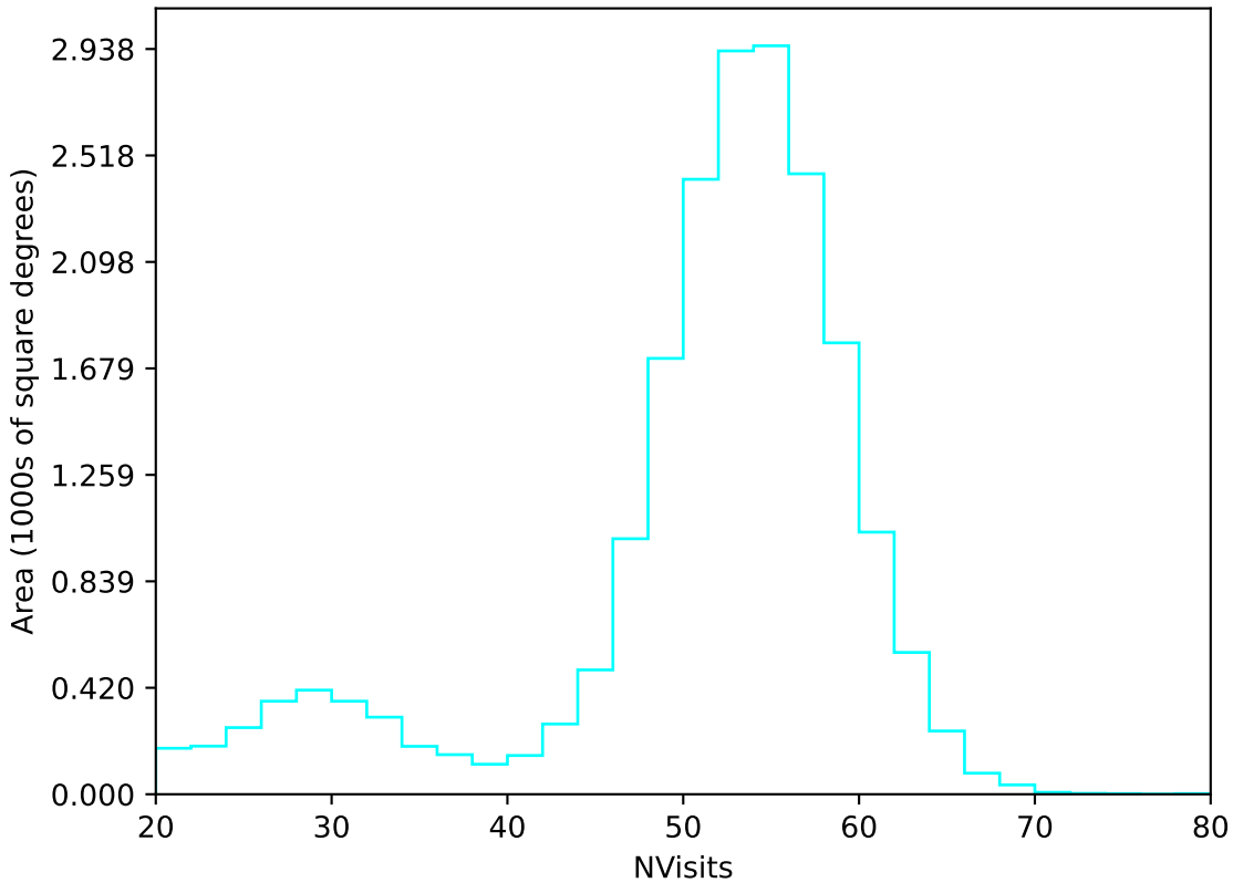
ddf_loaded_half_fl4_v3.4_10yrs All sky u band: NVisits
