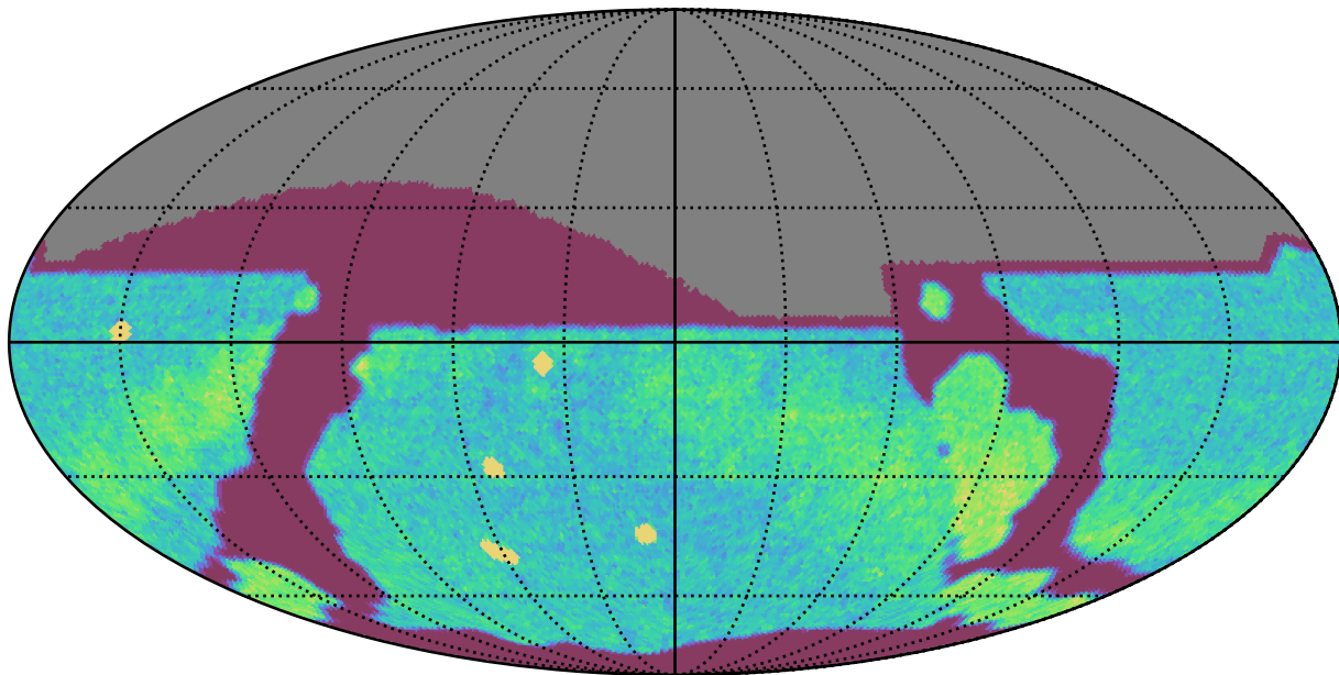
ddf_loaded_half_fl4_v3.4_10yrs All sky r band: NVisits
