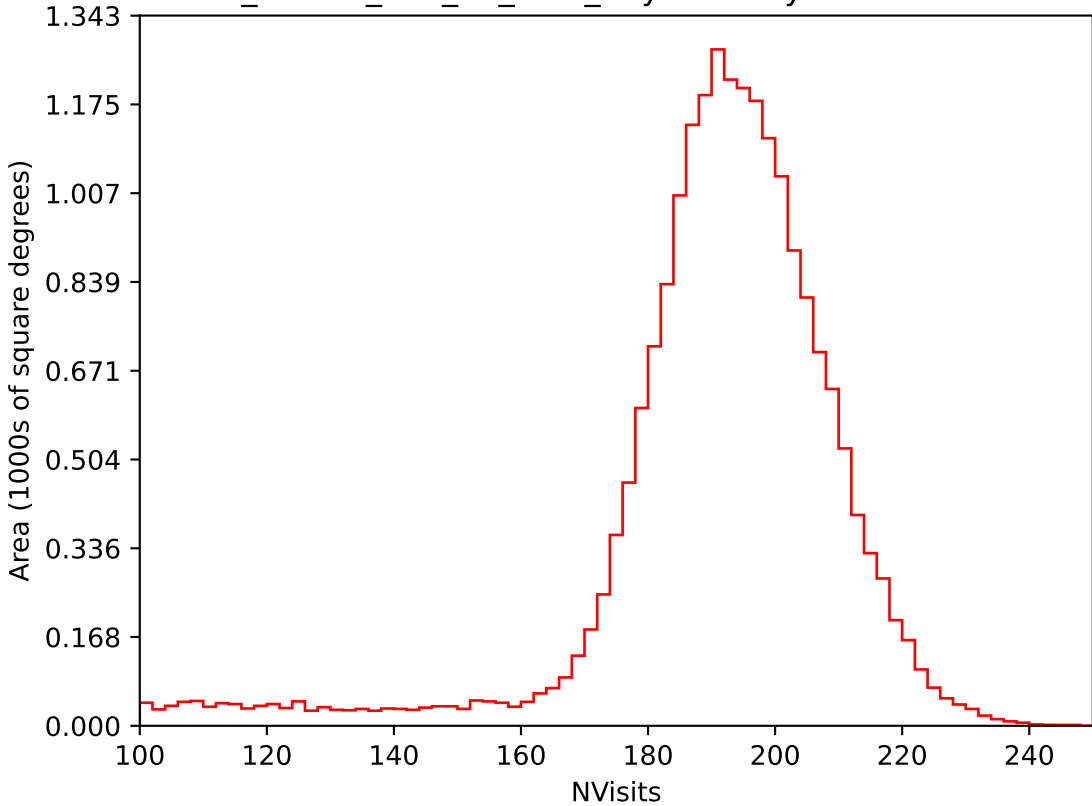
ddf_loaded_half_fl4_v3.4_10yrs All sky i band: NVisits
