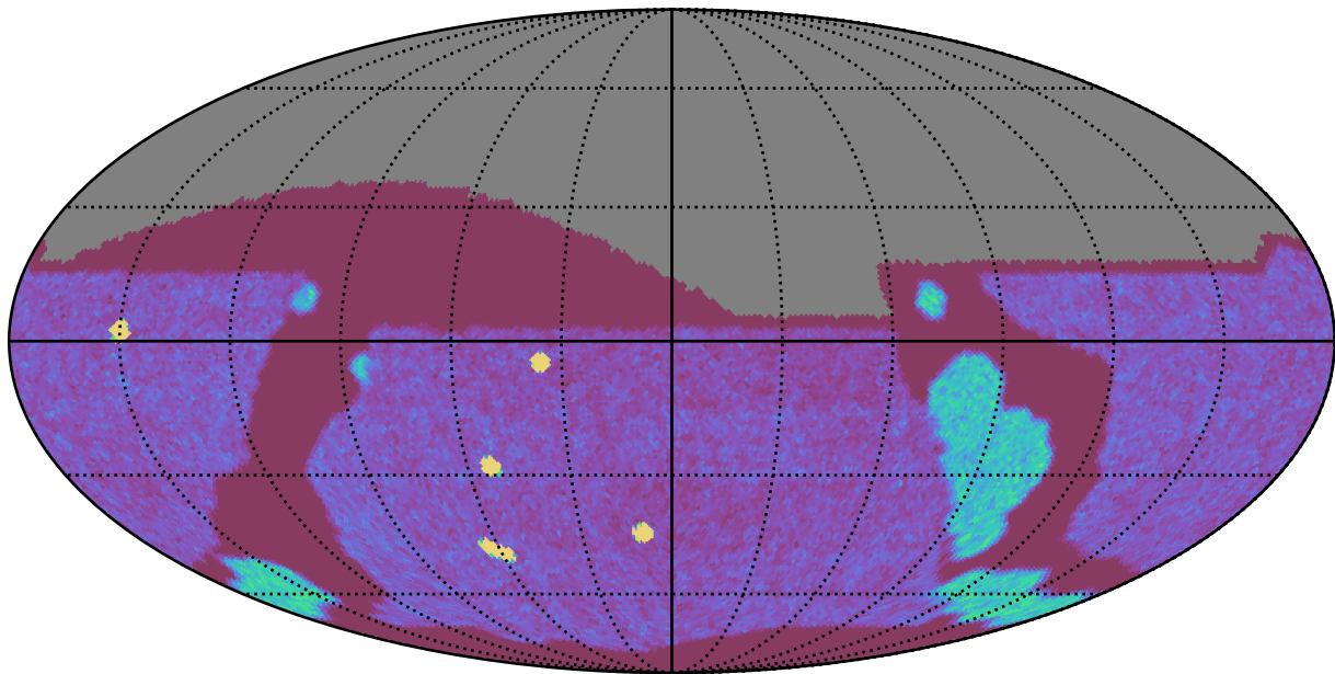
ddf_loaded_half_fl4_v3.4_10yrs All sky g band: NVisits
