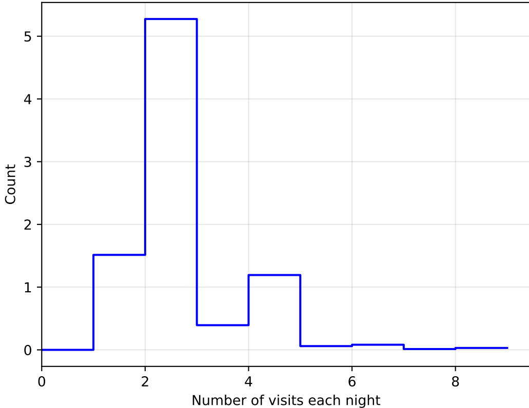
ddf_loaded_half_fl4_v3.4_10yrs WFD: NVisitsPerNight
