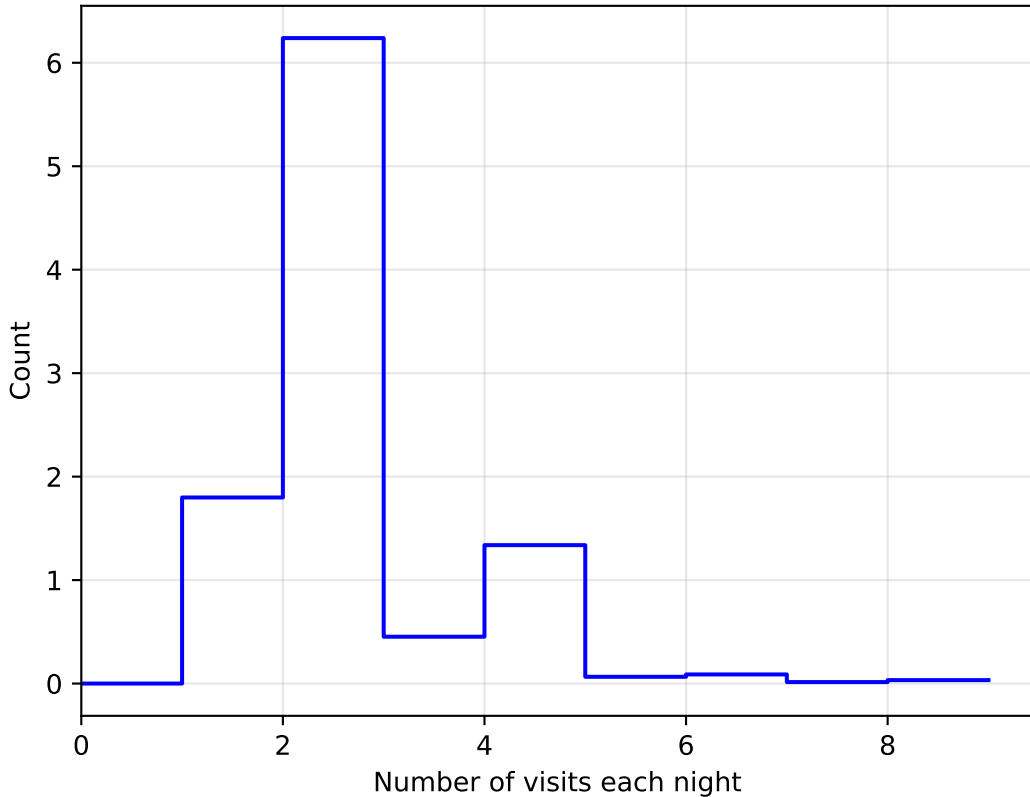
ddf_loaded_half_fl4_v3.4_10yrs All sky: NVisitsPerNight
