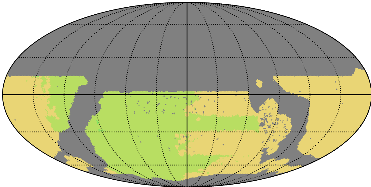
ddf_loaded_half_fl4_v3.4_10yrs WFD all bands: NSeasons
