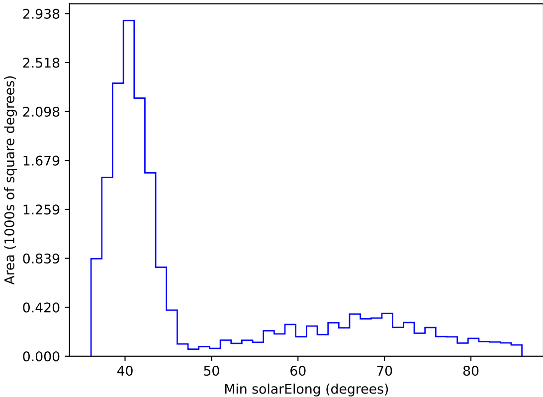
ddf_loaded_half_fl4_v3.4_10yrs WFD z band: Min solarElong
