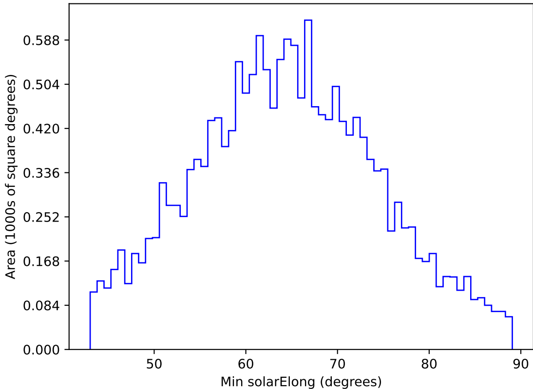
ddf_loaded_half_fl4_v3.4_10yrs WFD y band: Min solarElong
