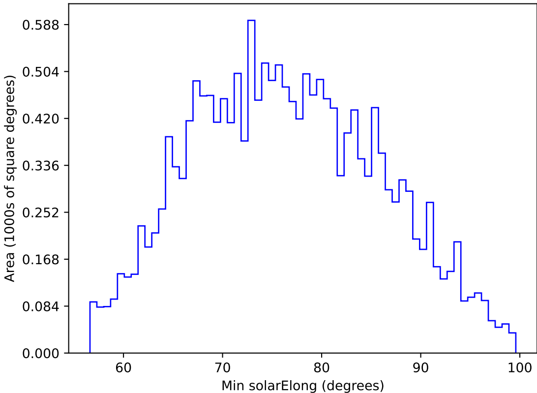
ddf_loaded_half_fl4_v3.4_10yrs WFD u band: Min solarElong
