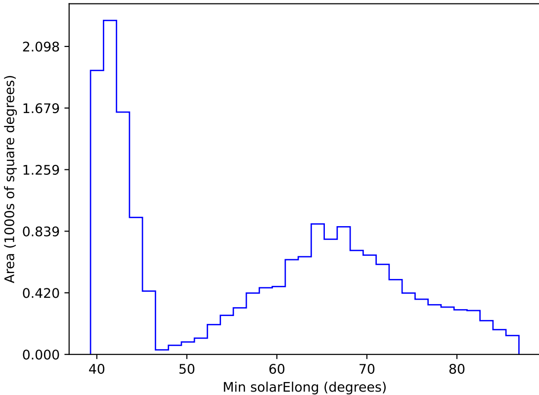
ddf_loaded_half_fl4_v3.4_10yrs WFD r band: Min solarElong
