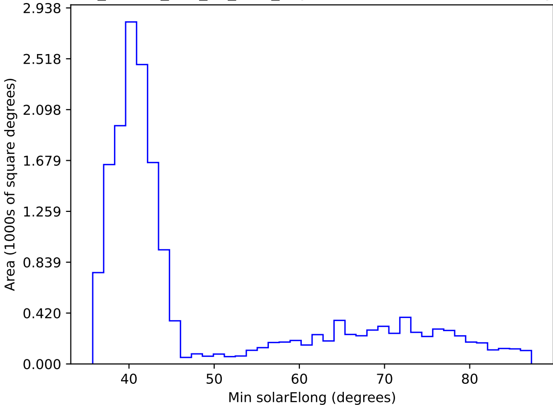
ddf_loaded_half_fl4_v3.4_10yrs WFD i band: Min solarElong
