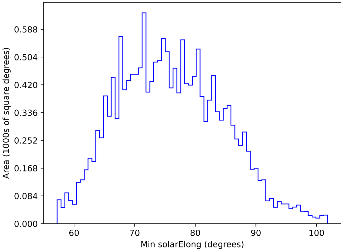
ddf_loaded_half_fl4_v3.4_10yrs WFD g band: Min solarElong
