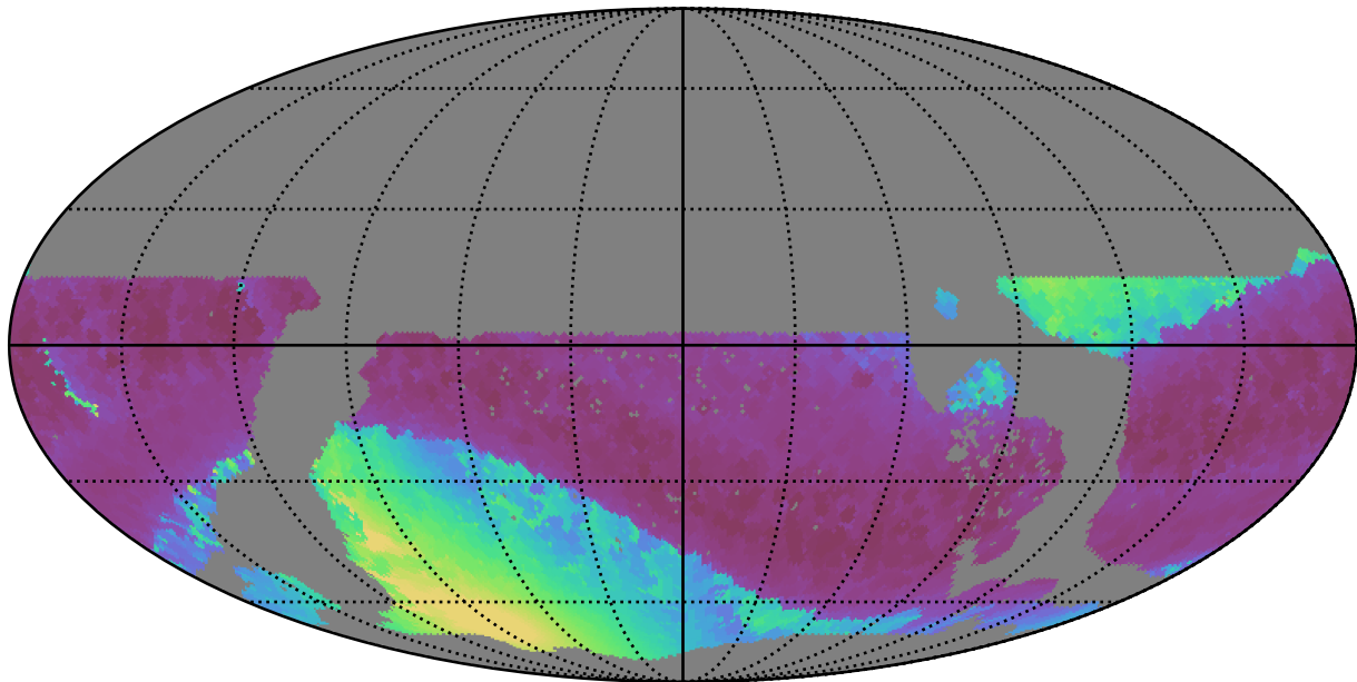
ddf_loaded_half_fl4_v3.4_10yrs WFD all bands: Min solarElong
