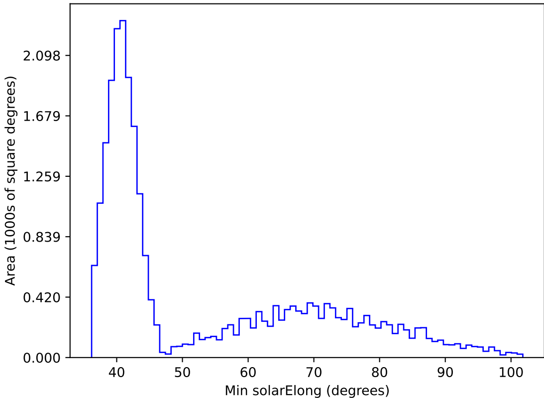
ddf_loaded_half_fl4_v3.4_10yrs All sky z band: Min solarElong
