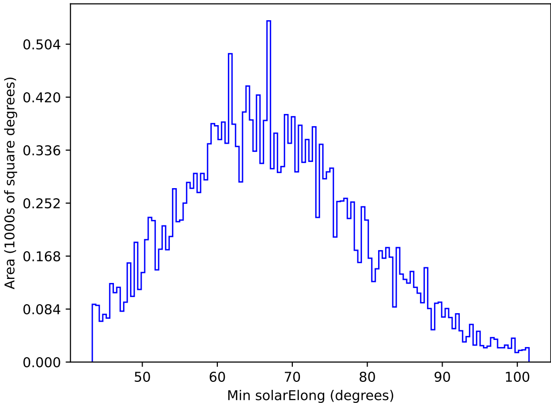
ddf_loaded_half_fl4_v3.4_10yrs All sky y band: Min solarElong
