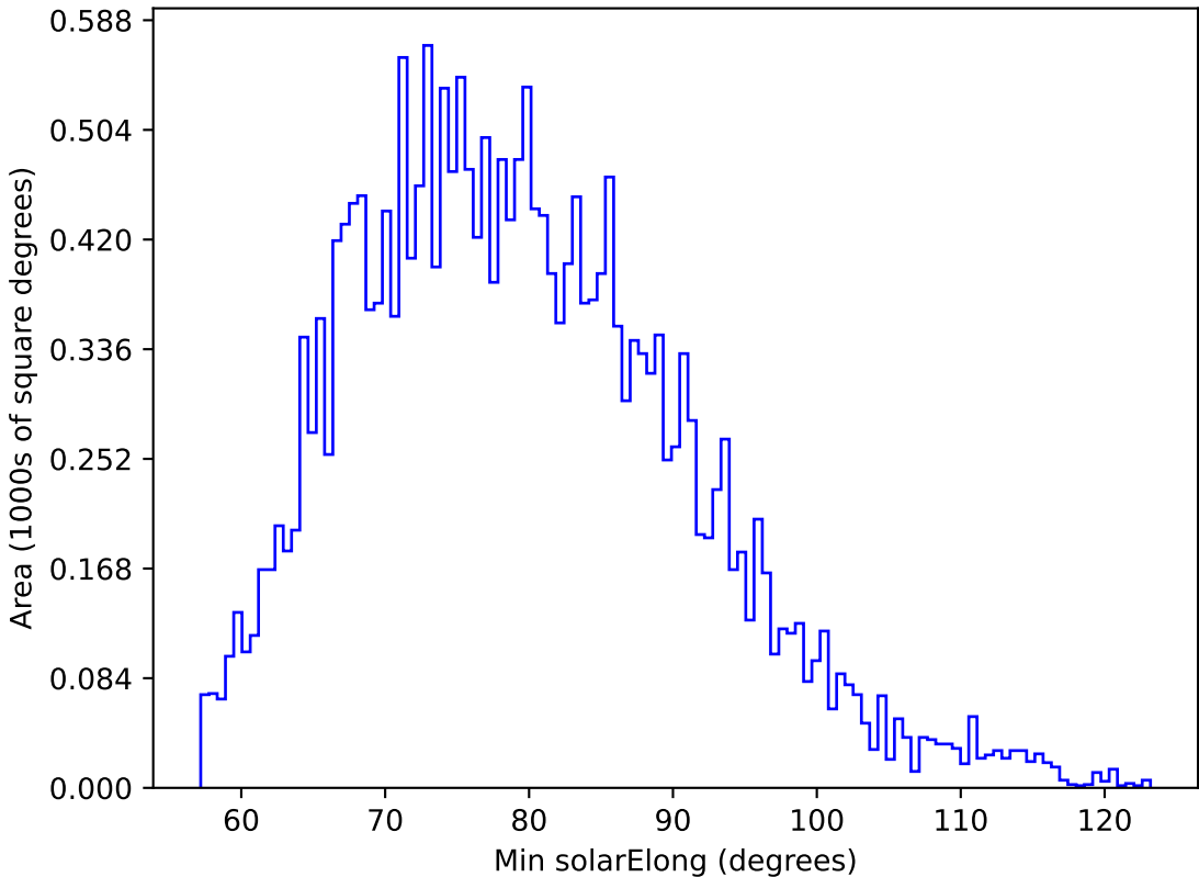
ddf_loaded_half_fl4_v3.4_10yrs All sky u band: Min solarElong
