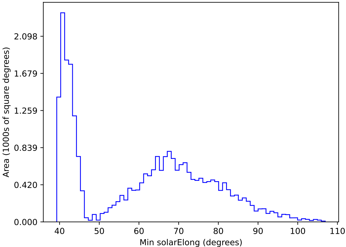
ddf_loaded_half_fl4_v3.4_10yrs All sky r band: Min solarElong
