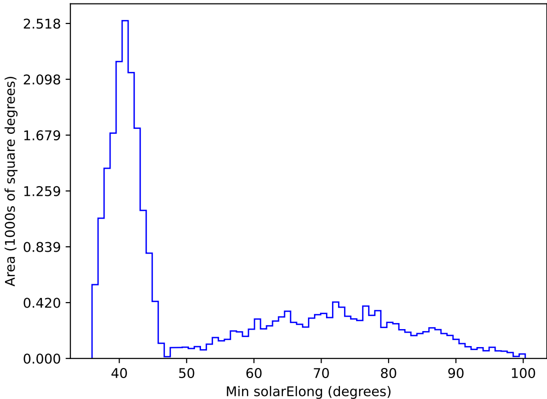
ddf_loaded_half_fl4_v3.4_10yrs All sky i band: Min solarElong
