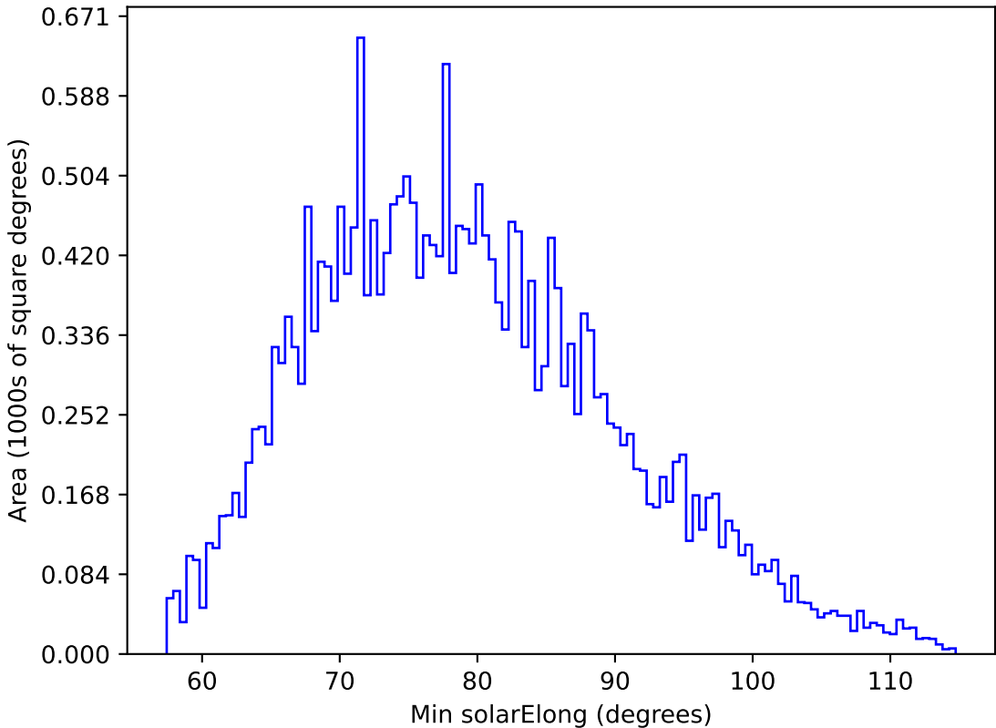
ddf_loaded_half_fl4_v3.4_10yrs All sky g band: Min solarElong
