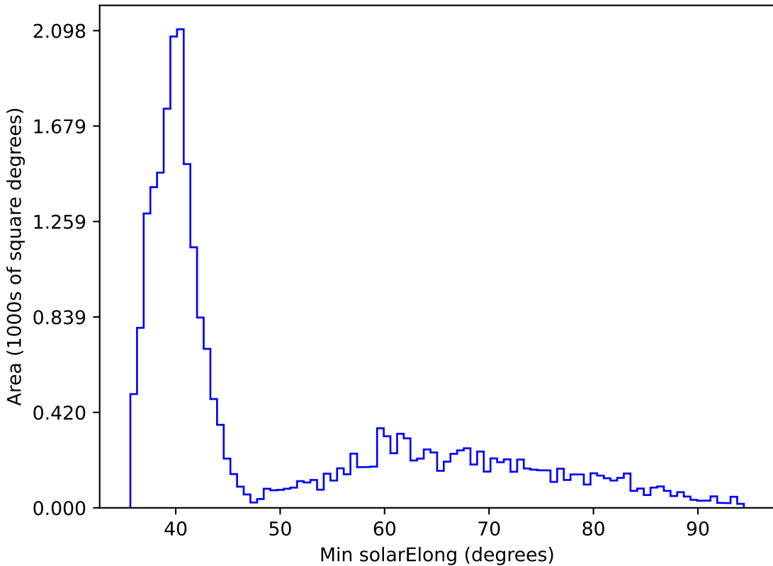
ddf_loaded_half_fl4_v3.4_10yrs All sky all bands: Min solarElong
