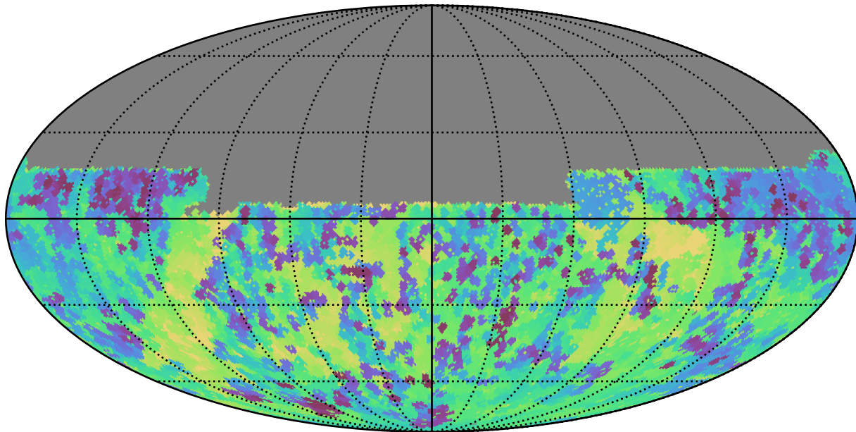
ddf_loaded_half_fl4_v3.4_10yrs Yr 1 y band: Min skyBrightness
