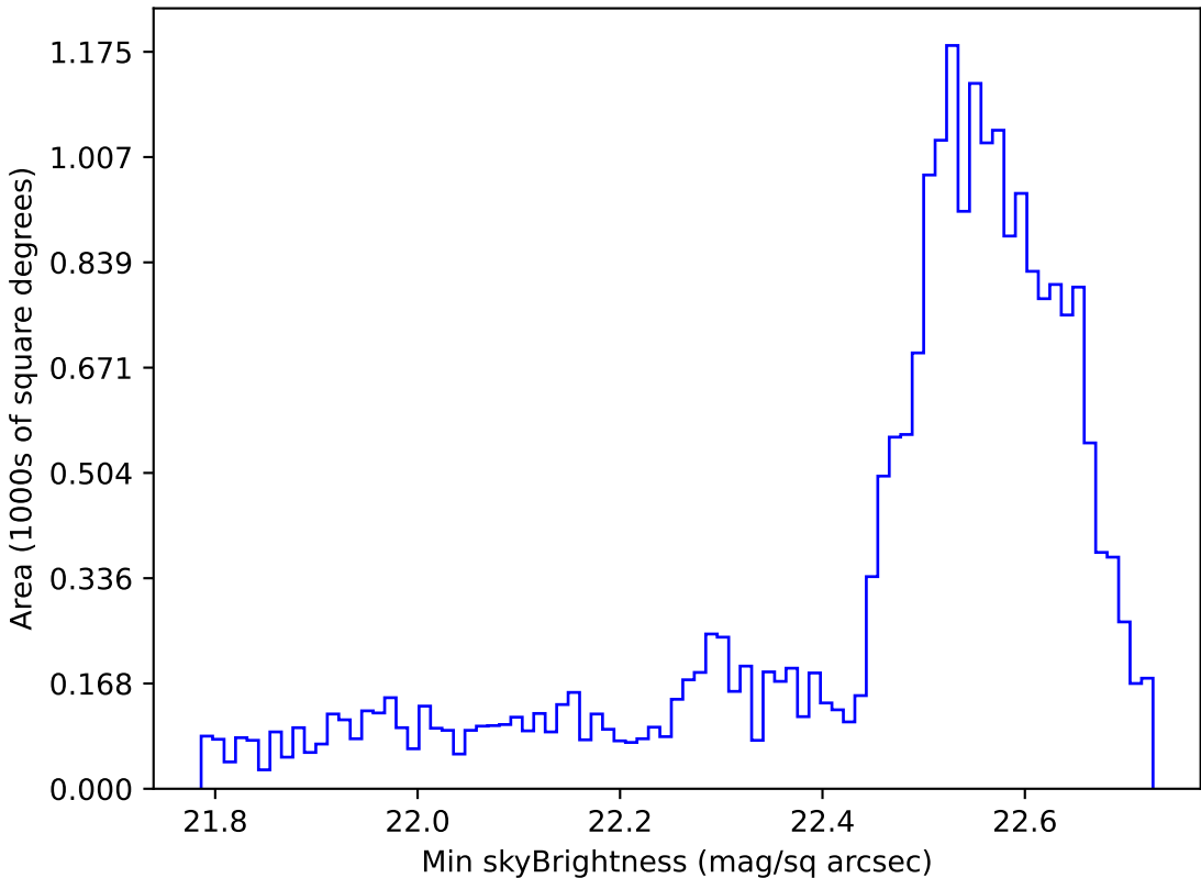
ddf_loaded_half_fl4_v3.4_10yrs Yr 1 u band: Min skyBrightness
