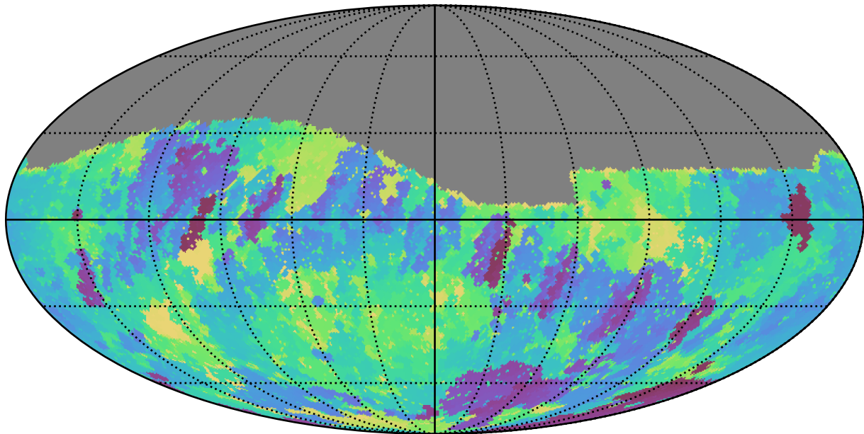
ddf_loaded_half_fl4_v3.4_10yrs Yr 1 r band: Min skyBrightness
