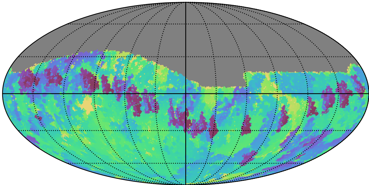
ddf_loaded_half_fl4_v3.4_10yrs Yr 1 i band: Min skyBrightness
