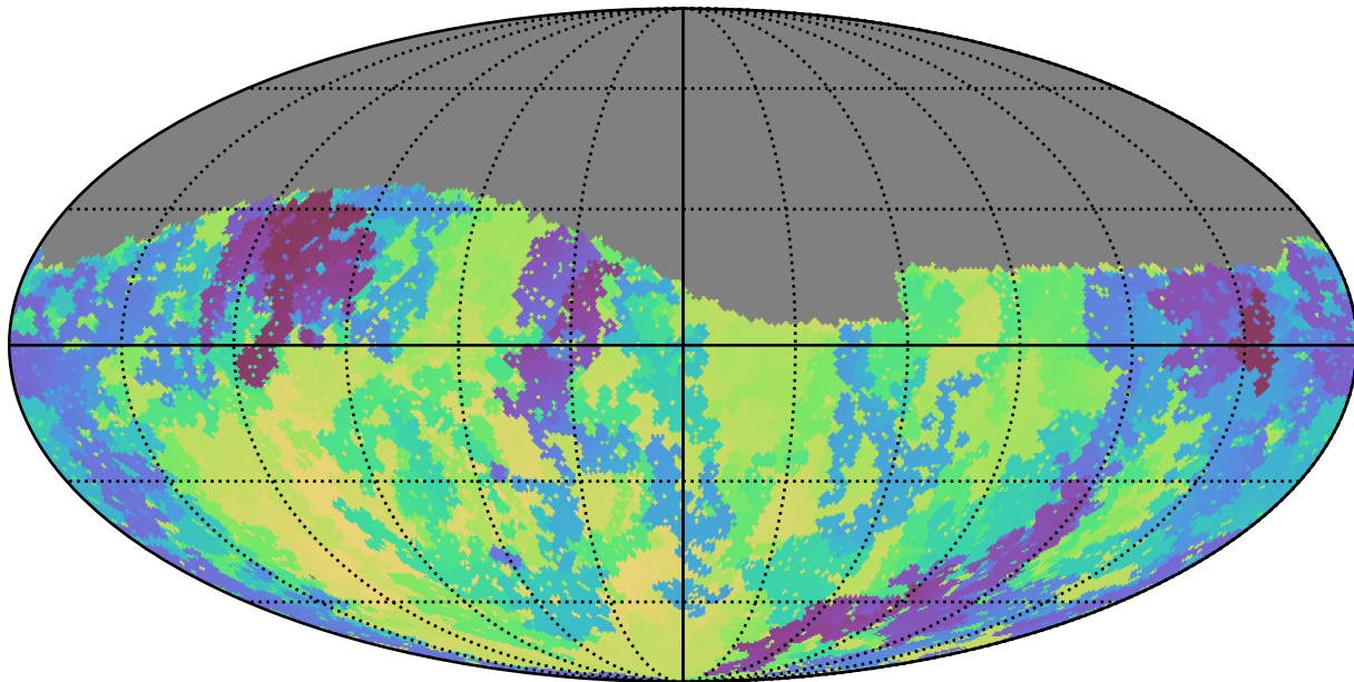
ddf_loaded_half_fl4_v3.4_10yrs Yr 1 g band: Min skyBrightness
