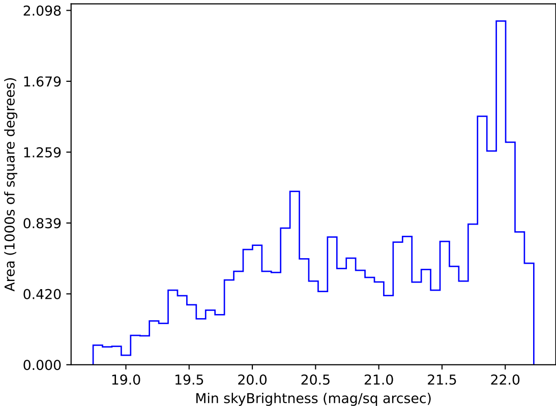
ddf_loaded_half_fl4_v3.4_10yrs Yr 1 g band: Min skyBrightness
