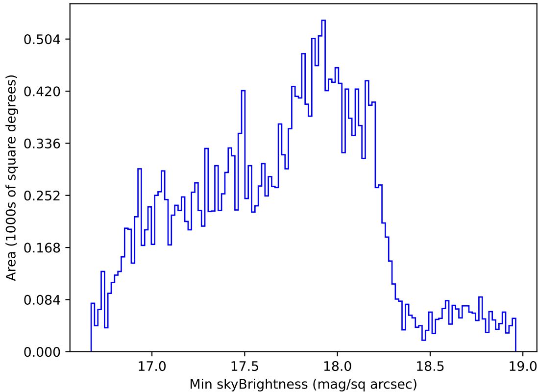
ddf_loaded_half_fl4_v3.4_10yrs Yr 1 all bands: Min skyBrightness
