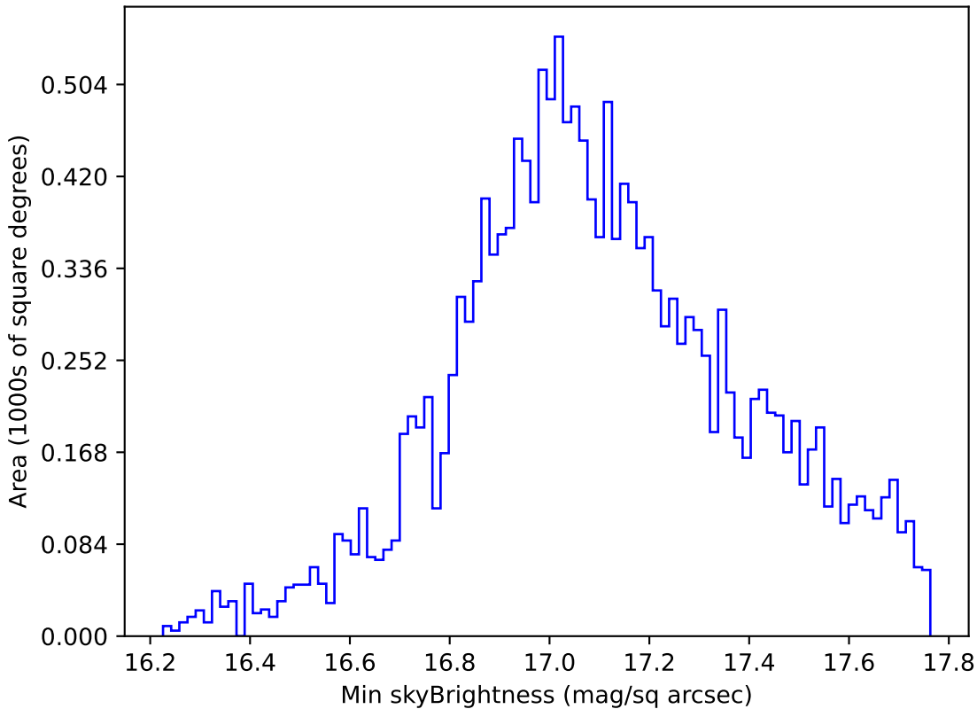
ddf_loaded_half_fl4_v3.4_10yrs WFD y band: Min skyBrightness
