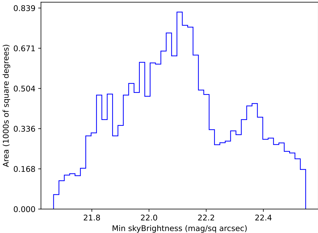
ddf_loaded_half_fl4_v3.4_10yrs WFD u band: Min skyBrightness
