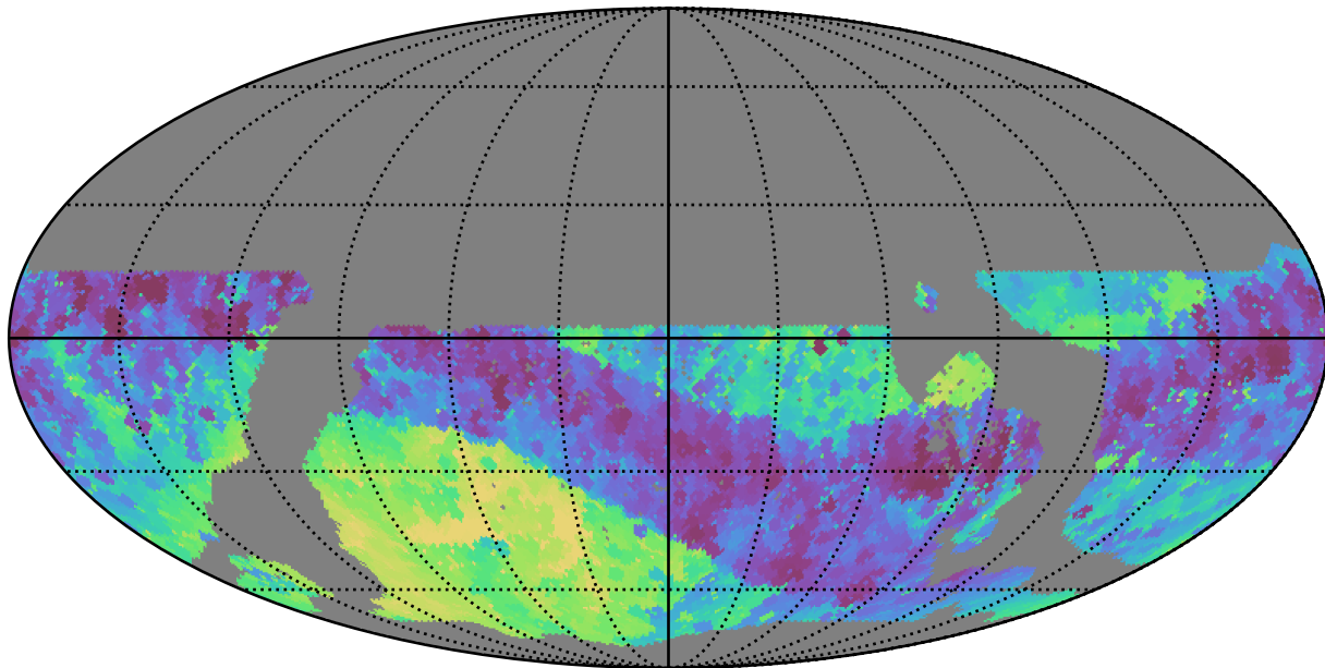
ddf_loaded_half_fl4_v3.4_10yrs WFD i band: Min skyBrightness
