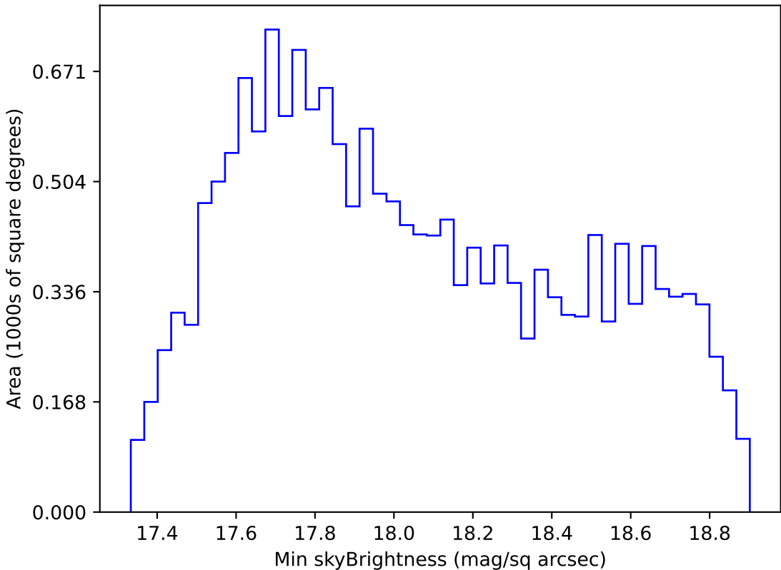
ddf_loaded_half_fl4_v3.4_10yrs WFD i band: Min skyBrightness
