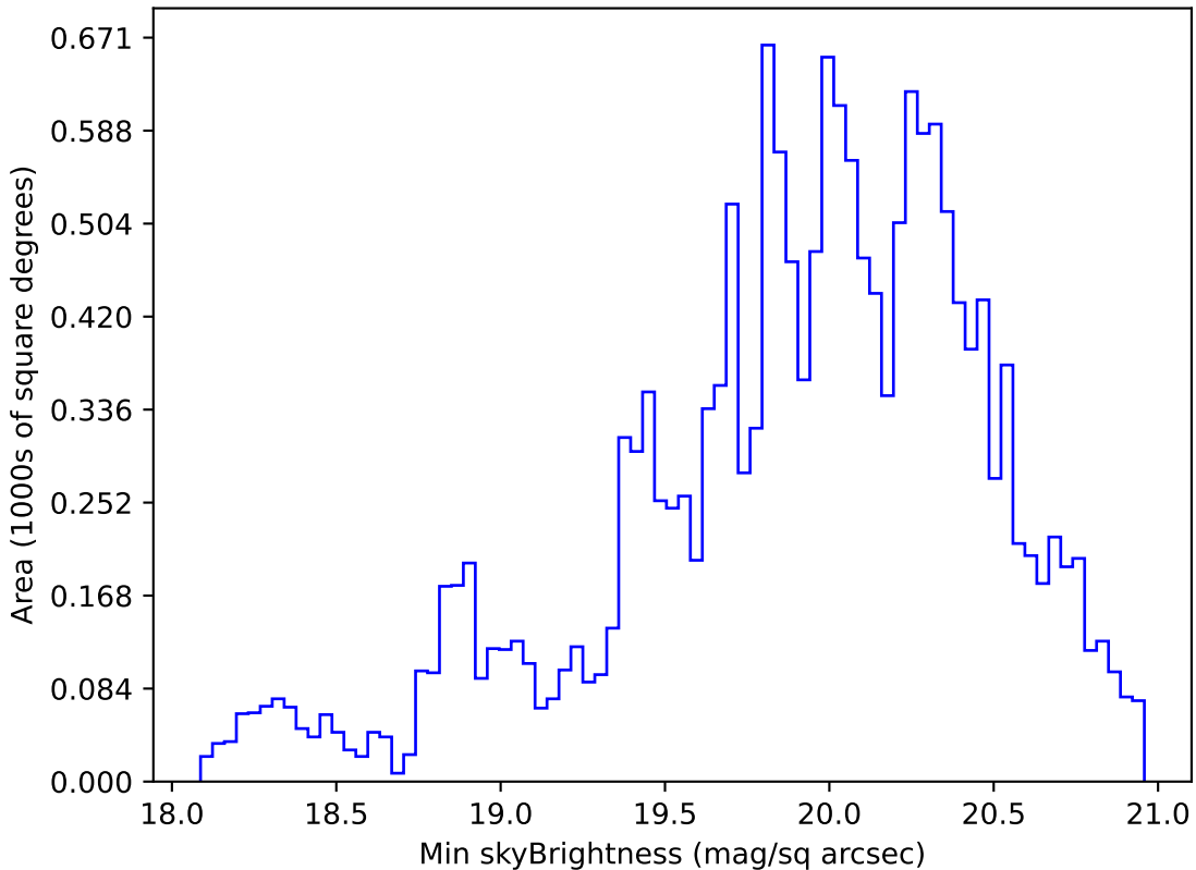
ddf_loaded_half_fl4_v3.4_10yrs WFD g band: Min skyBrightness
