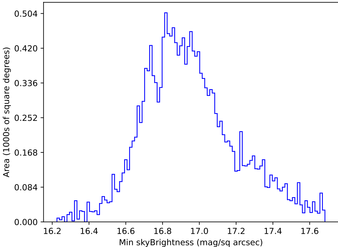
ddf_loaded_half_fl4_v3.4_10yrs WFD all bands: Min skyBrightness
