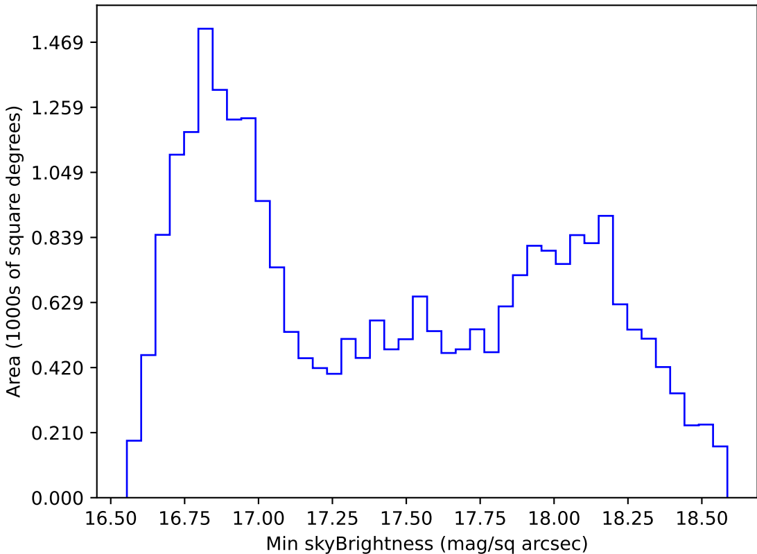
ddf_loaded_half_fl4_v3.4_10yrs All sky z band: Min skyBrightness
