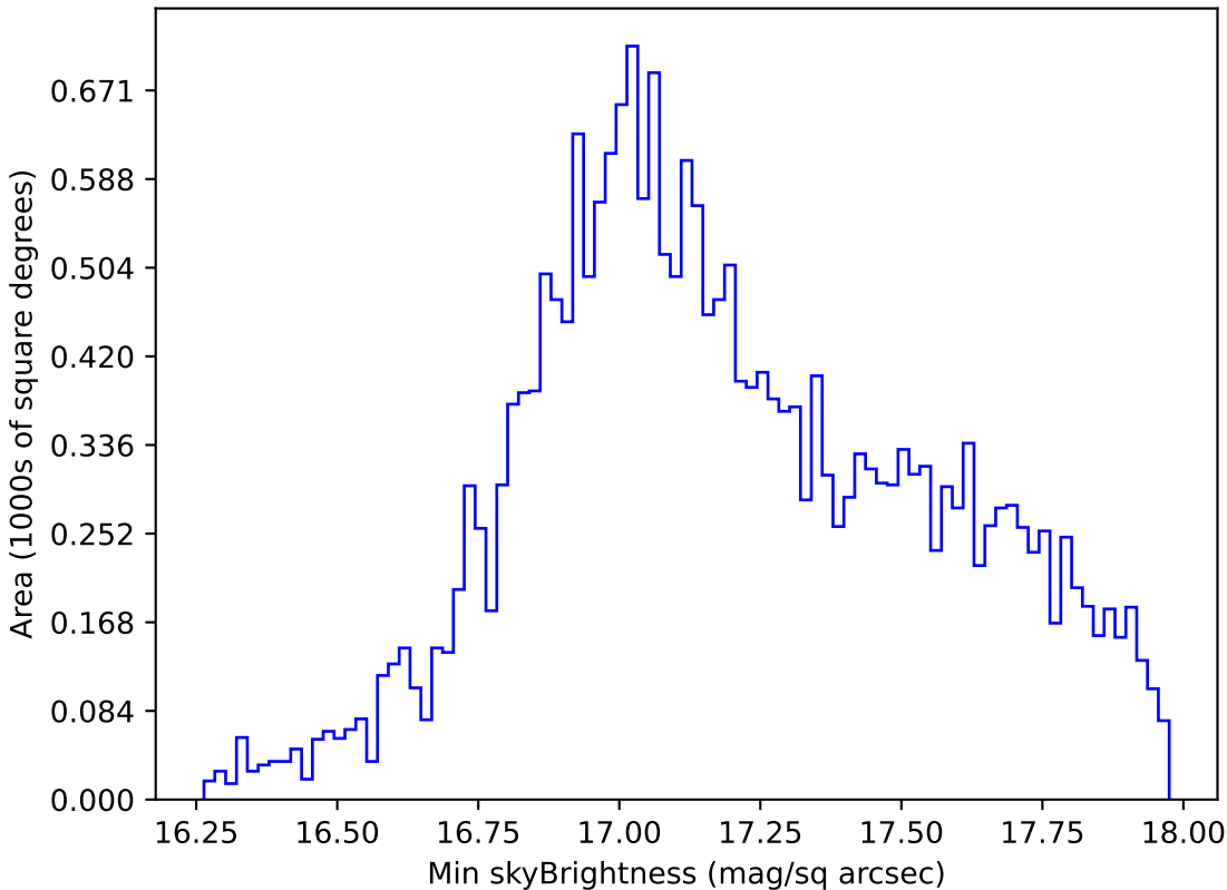
ddf_loaded_half_fl4_v3.4_10yrs All sky y band: Min skyBrightness
