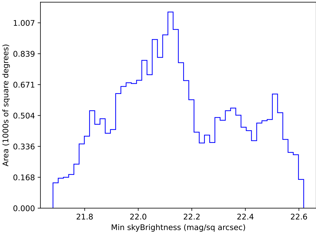
ddf_loaded_half_fl4_v3.4_10yrs All sky u band: Min skyBrightness
