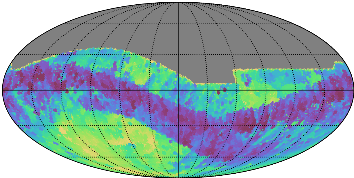
ddf_loaded_half_fl4_v3.4_10yrs All sky i band: Min skyBrightness
