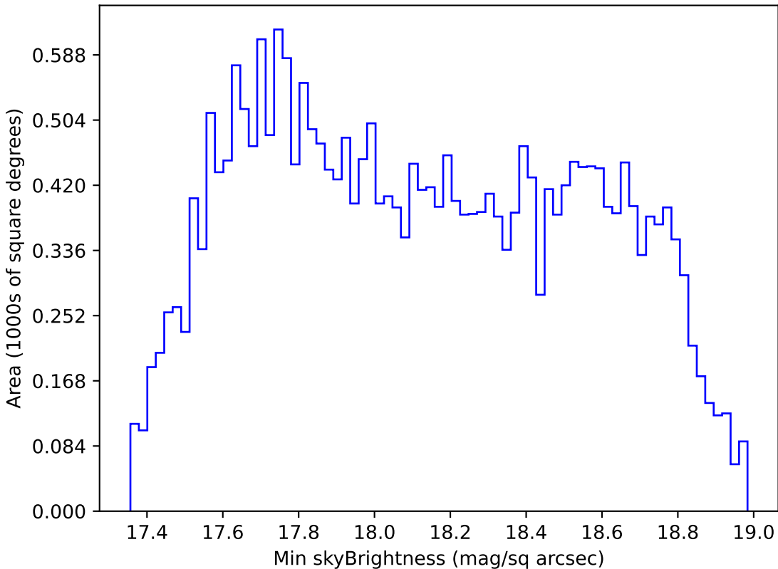
ddf_loaded_half_fl4_v3.4_10yrs All sky i band: Min skyBrightness
