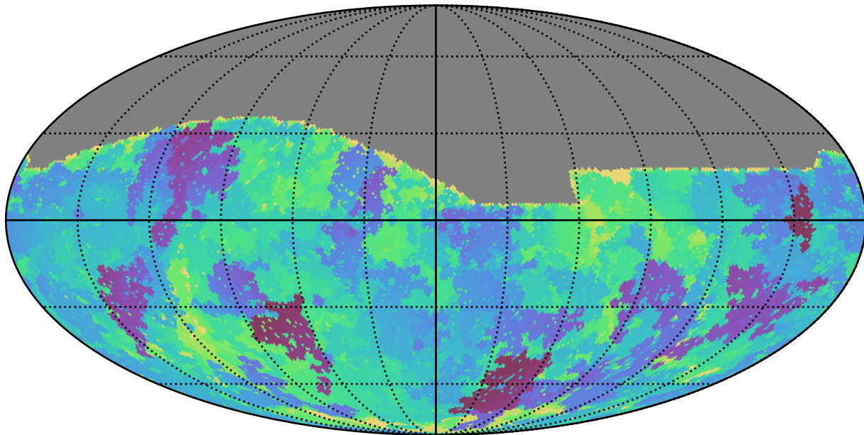
ddf_loaded_half_fl4_v3.4_10yrs All sky g band: Min skyBrightness
