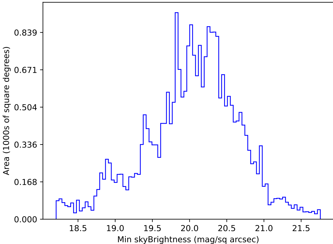
ddf_loaded_half_fl4_v3.4_10yrs All sky g band: Min skyBrightness
