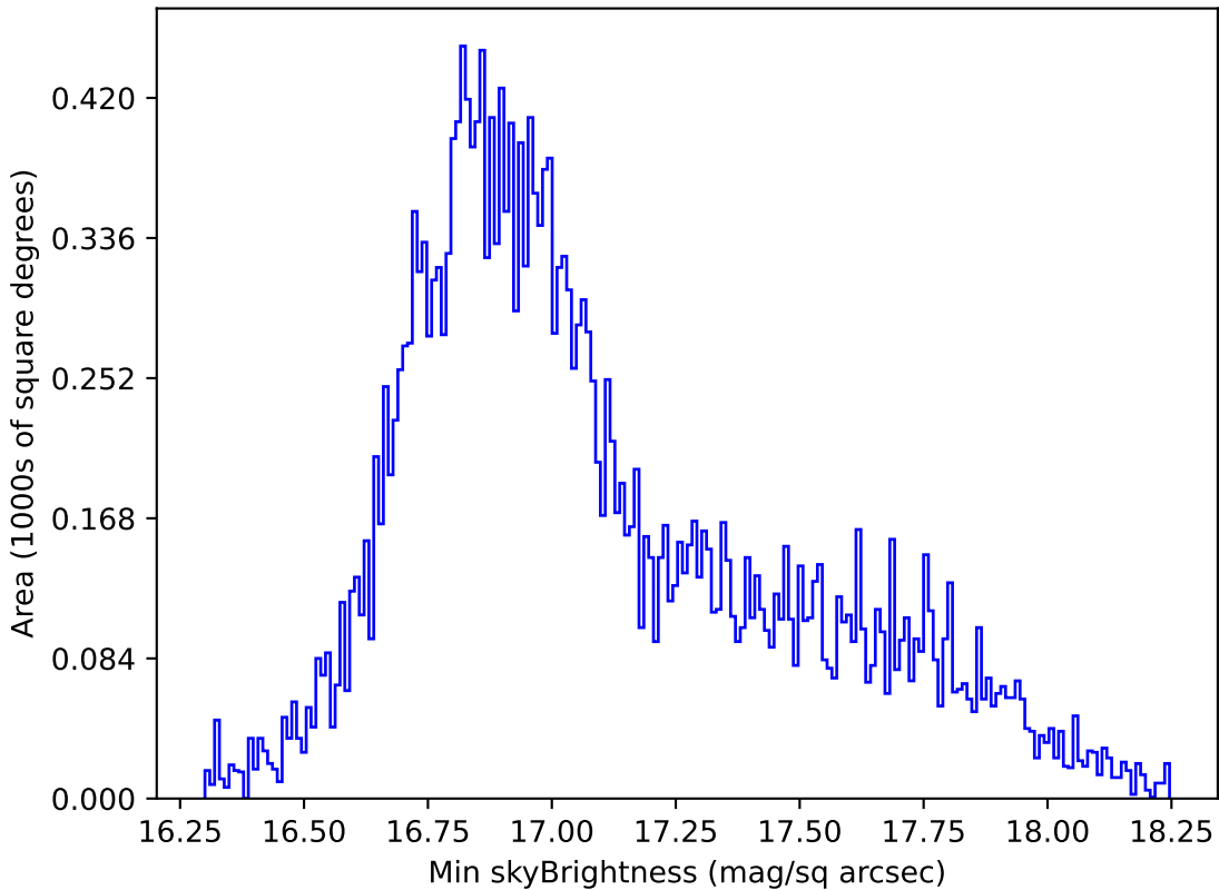
ddf_loaded_half_fl4_v3.4_10yrs All sky all bands: Min skyBrightness
