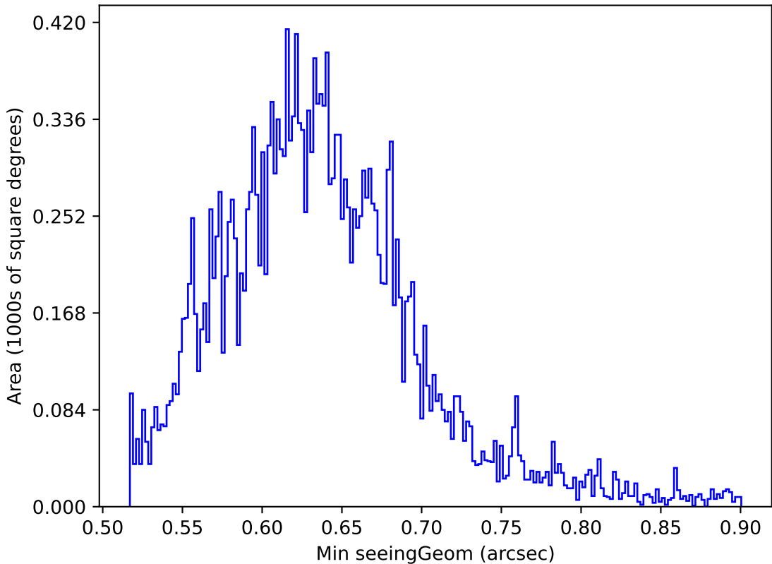
ddf_loaded_half_f14_v3.4_10yrs Yr 1 y band: Min seeingGeom
