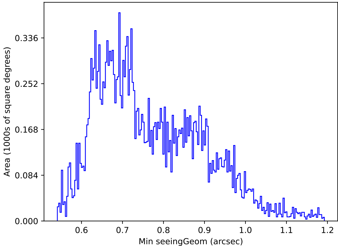
ddf_loaded_half_fl4_v3.4_10yrs Yr 1 u band: Min seeingGeom
