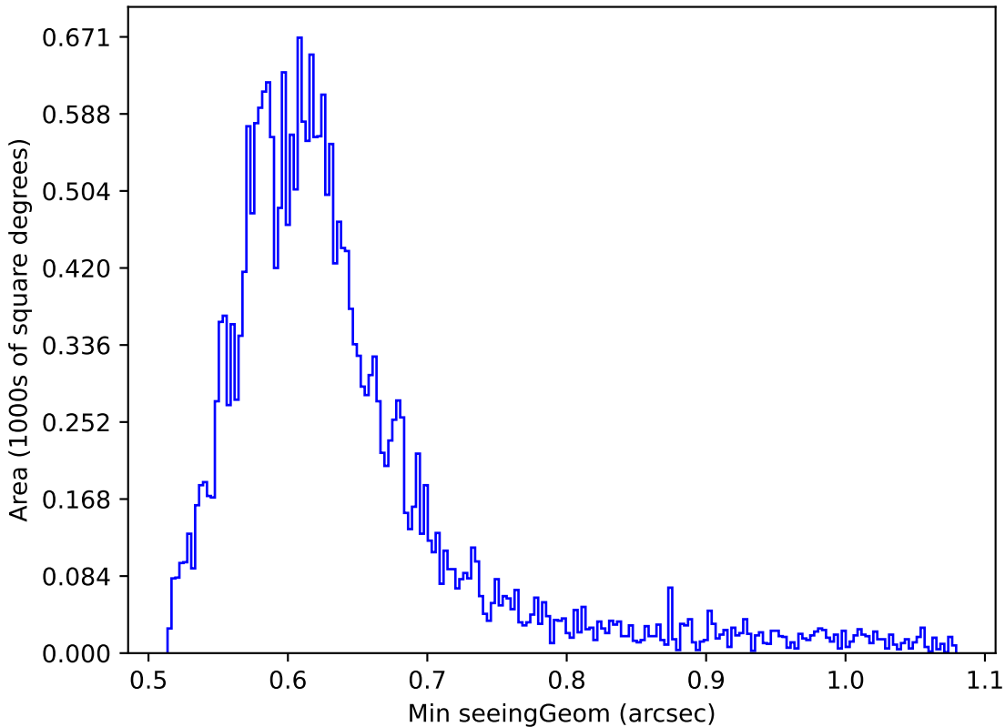
ddf_loaded_half_fl4_v3.4_10yrs Yr 1 r band: Min seeingGeom
