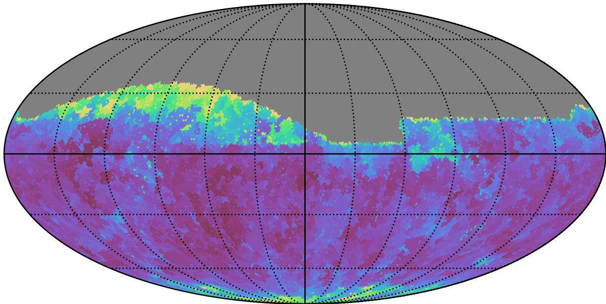
ddf_loaded_half_fl4_v3.4_10yrs Yr 1 i band: Min seeingGeom
