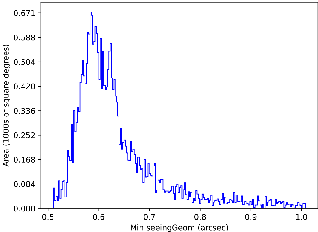
ddf_loaded_half_fl4_v3.4_10yrs Yr 1 i band: Min seeingGeom
