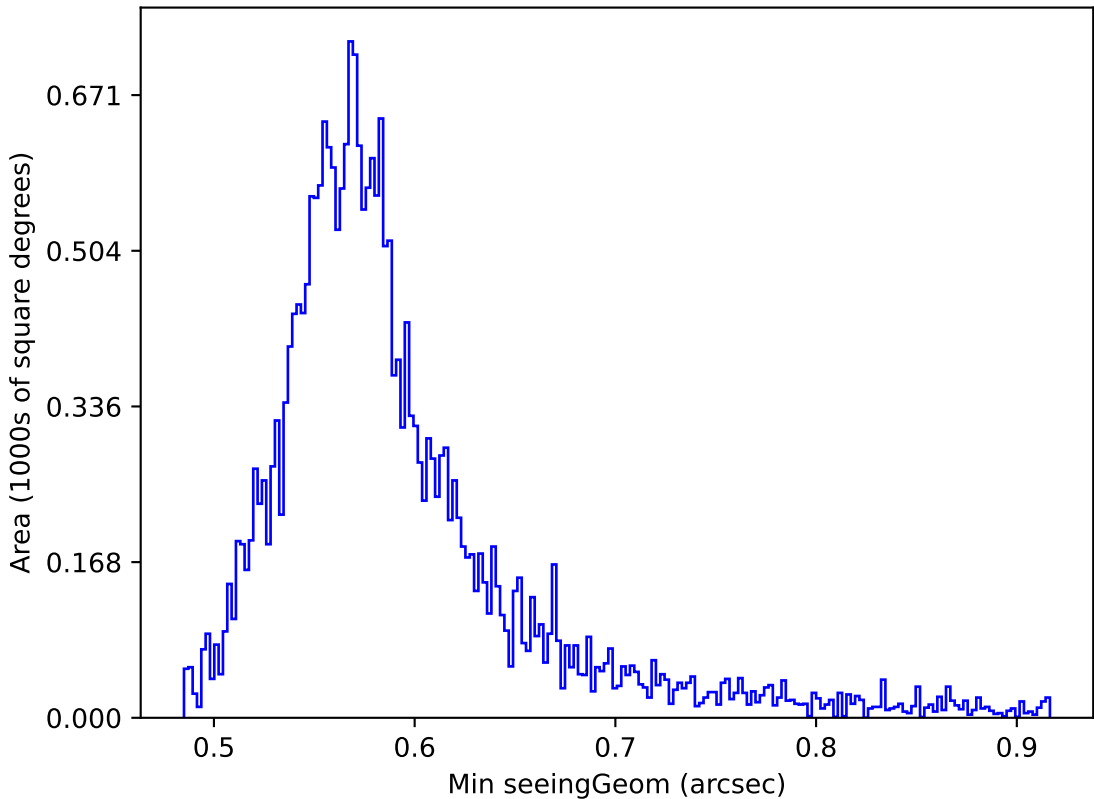
ddf_loaded_half_fl4_v3.4_10yrs Yr 1 all bands: Min seeingGeom
